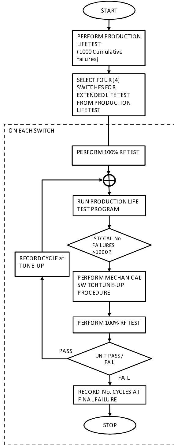
Figure 6 – Extended Life Test Data (with Tune-up) Process Flow
