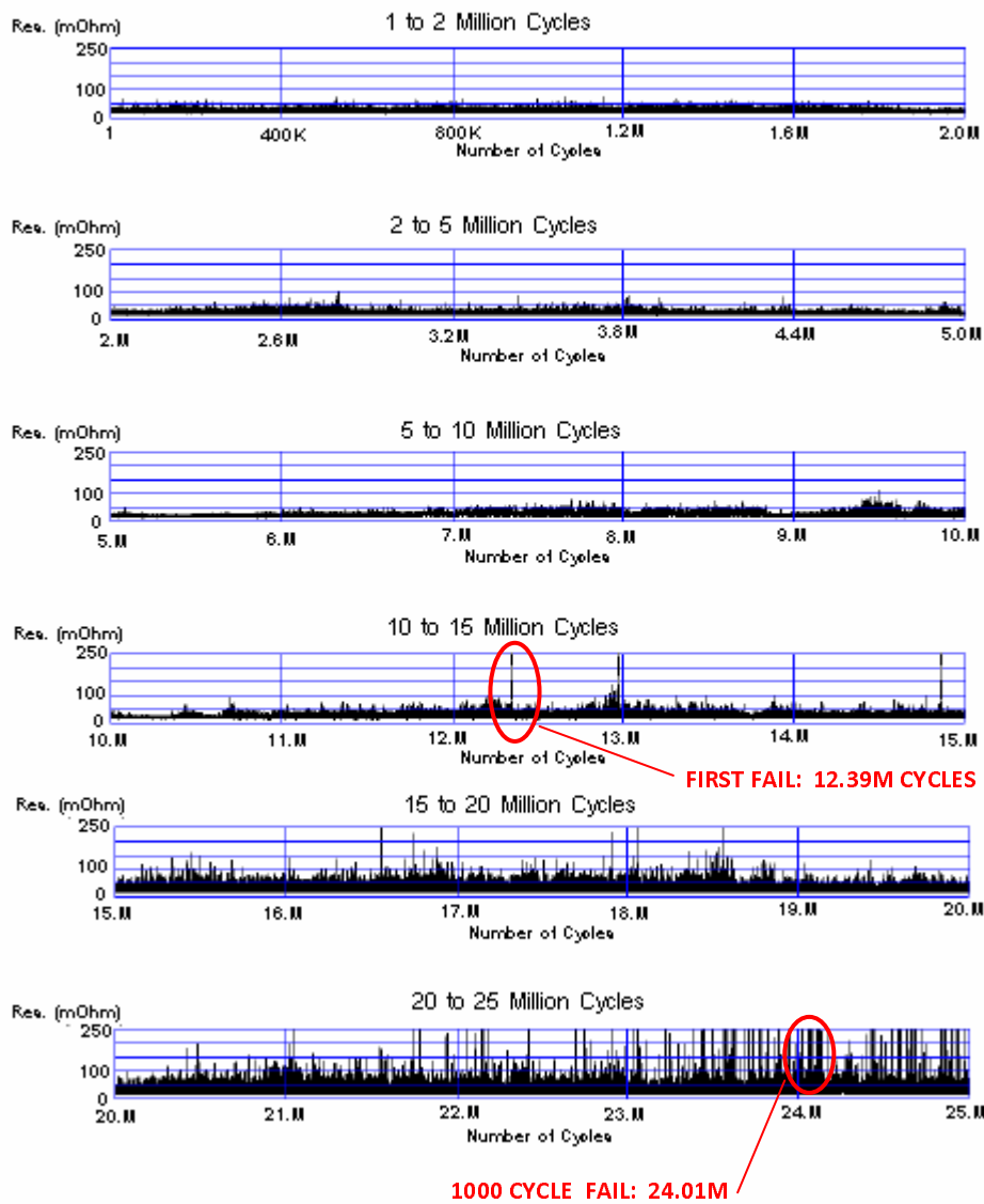
Figure 3 – Sample Life Test Data – one Switch
