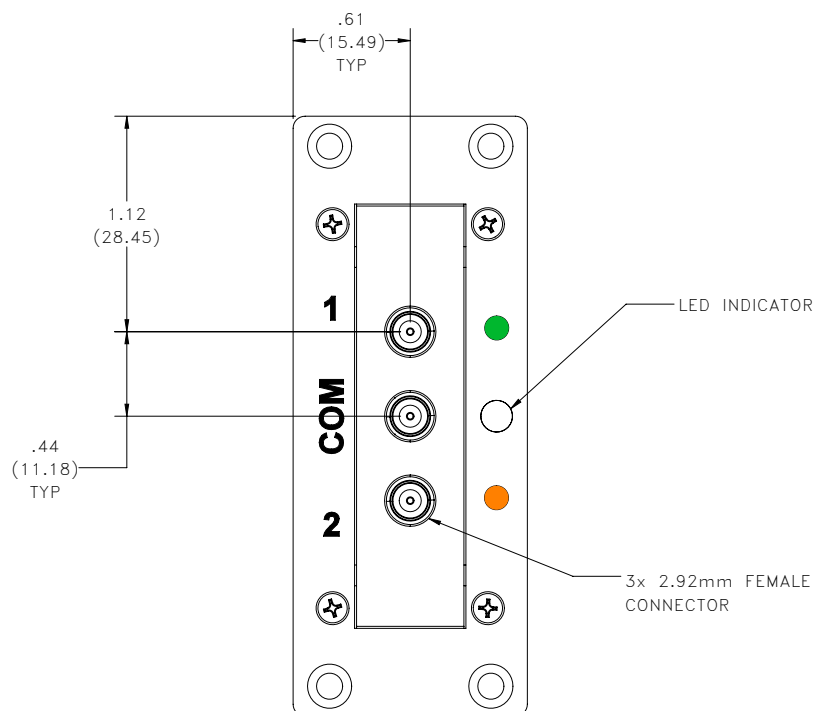
SPDTA-40GHz
