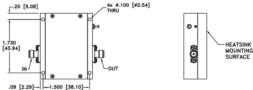
MOUNTING INFORMATION OF MODEL WITHOUT HEATSINK
