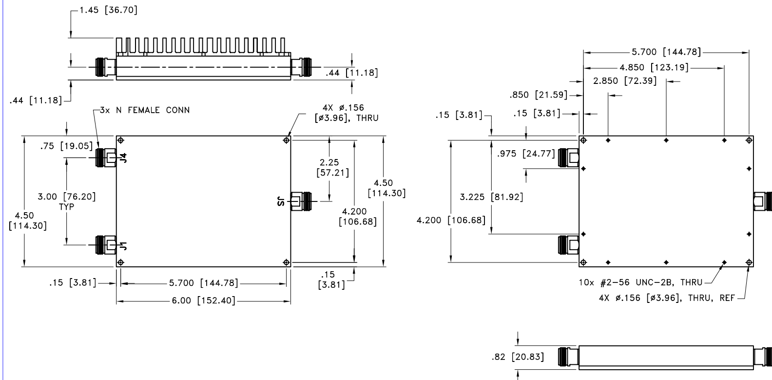
MOUNTING INFORMATION FOR MODEL WITHOUT HEATSINK
