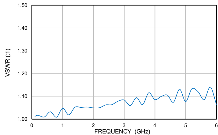
N Female Bulkhead VSWR (+25°C)
