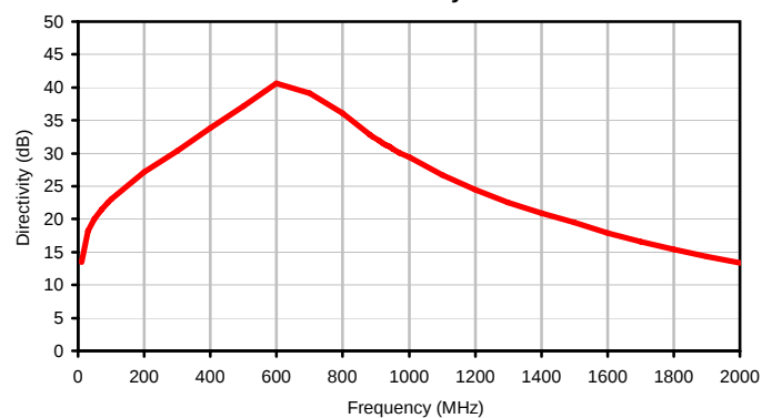
Directivity
