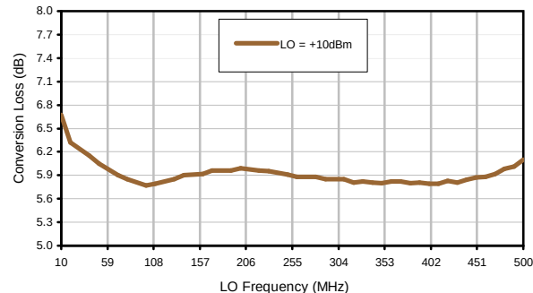
Conversion Loss @ RF=510.1 MHz
