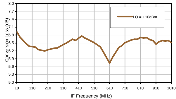
Conversion Loss vs. IF @ RF=1210.9 MHz
