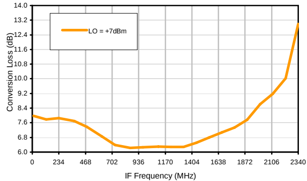
Conversion Loss vs. IF @ RF=3500.1001MHz
