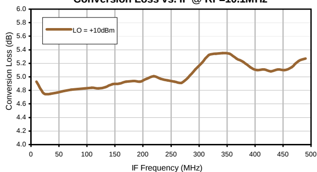
Conversion Loss vs. IF @ RF=10.1MHz
