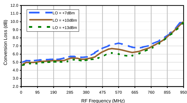
Conversion Loss @ IF=30MHz
