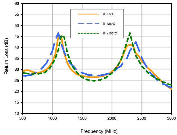
Return Loss Reverse vs. TEMPERATURE
