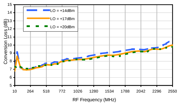
Conversion Loss @ IF=413MHz
