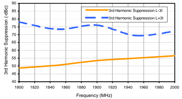
3rd Harmonic Suppression
