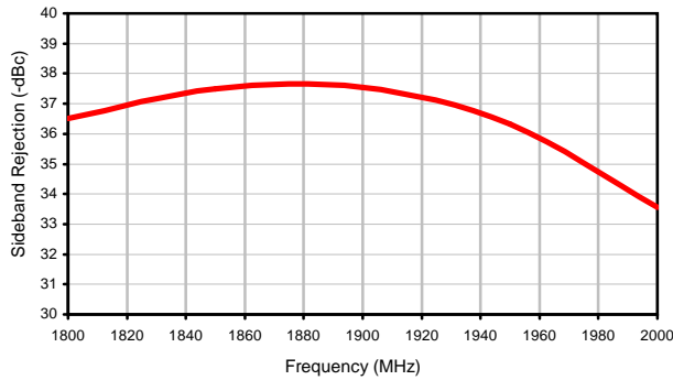
Sideband Rejection LSB
