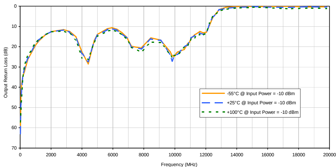
OUTPUT RETURN LOSS vs. TEMPERATURE
