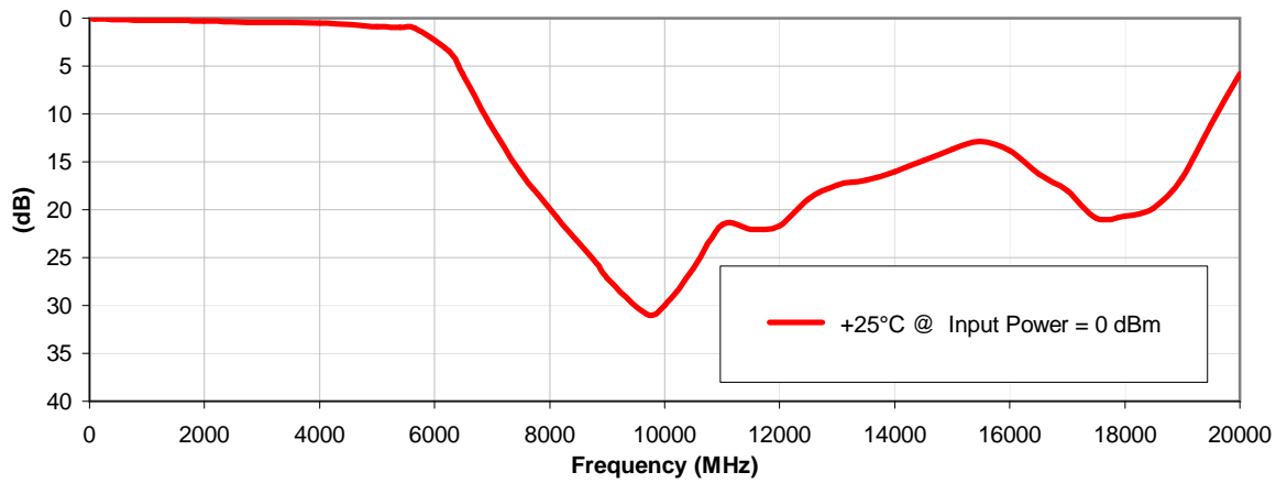
INSERTION LOSS
