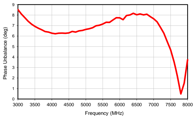
Phase Unbalance
