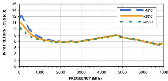
INPUT RETURN LOSS vs. FREQUENCY & TEMPERATURE Vd = 3V, Rbias=1K Ohms
