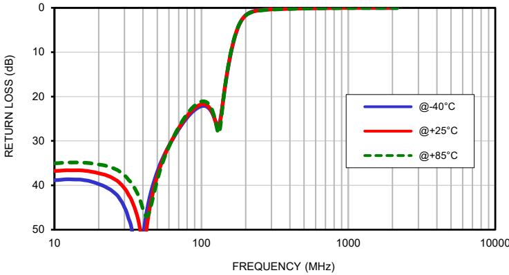
COMMON PORT vs. TEMPERATURE INPUT POWER = 0 dBm
