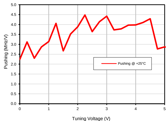
Frequency Pushing
