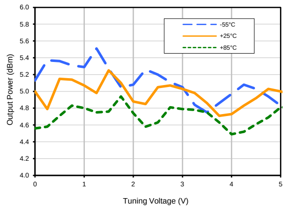
Power Output
