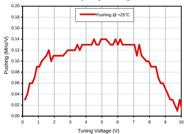
Frequency Pushing
