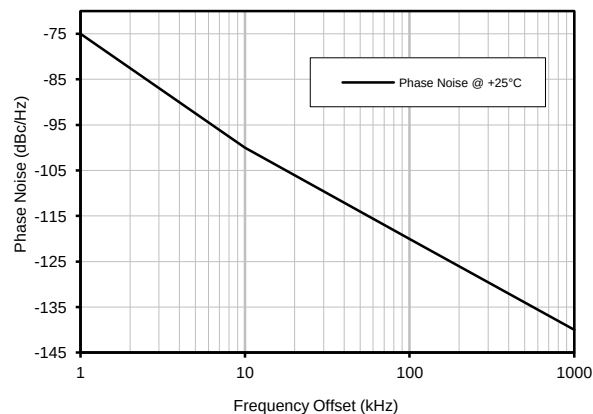
Phase Noise
