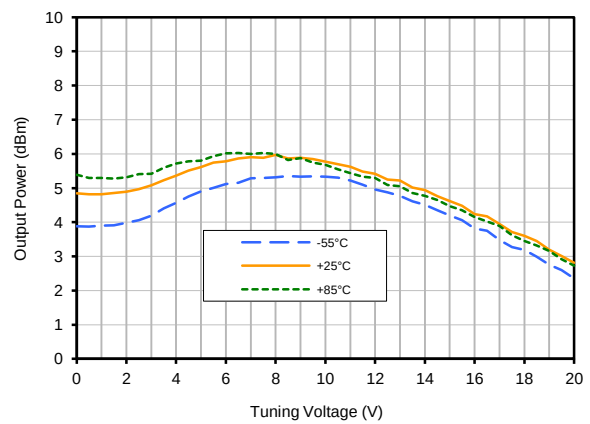
Output Power
