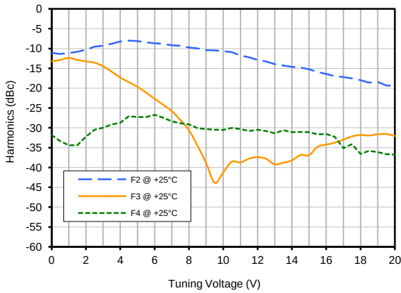
Harmonics Level
