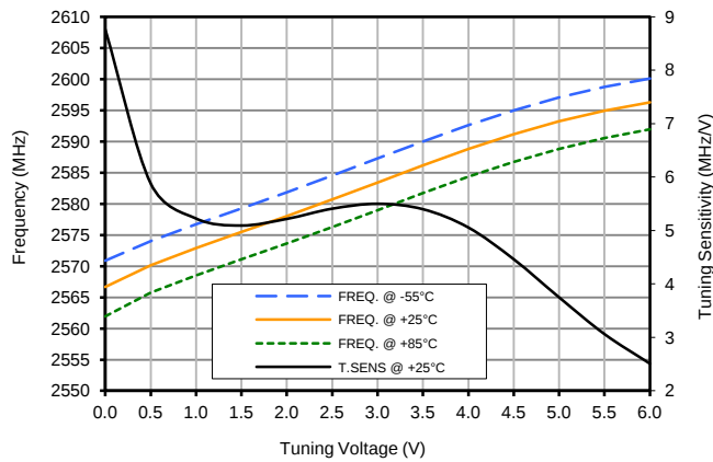
Frequency and Tuning Sensitivity
