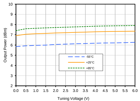
Output Power
