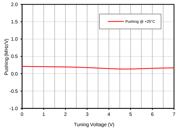
Frequency Pushing
