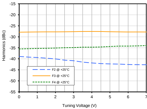
Harmonics Level
