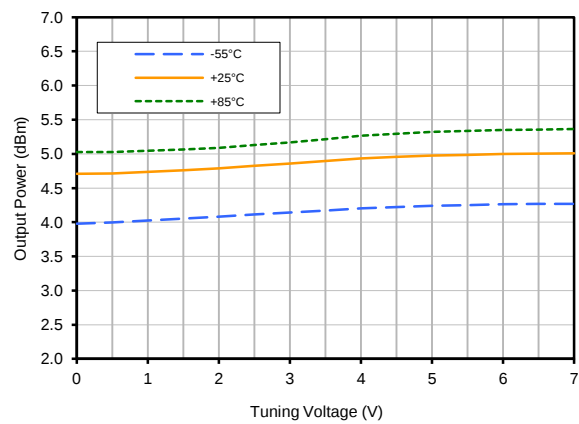
Output Power
