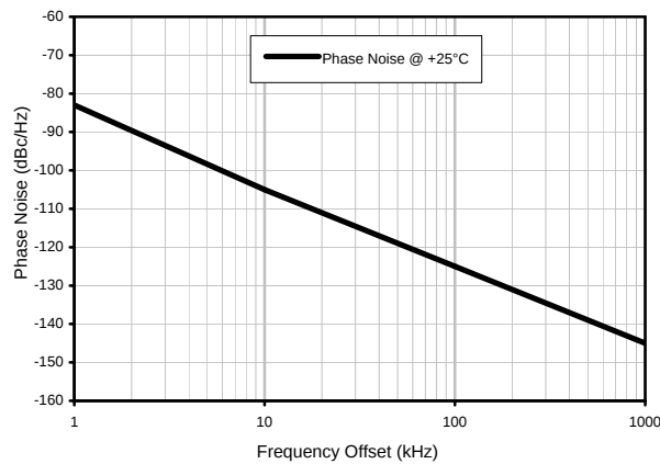
Phase Noise
