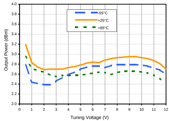
Power Output
