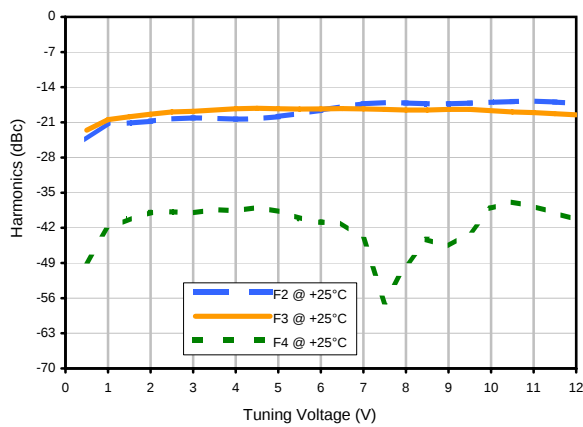
Harmonics Level
