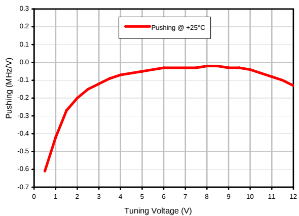
Frequency Pushing
