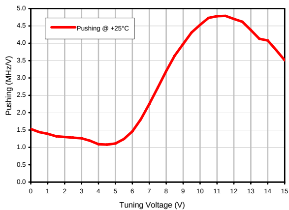
Frequency Pushing
