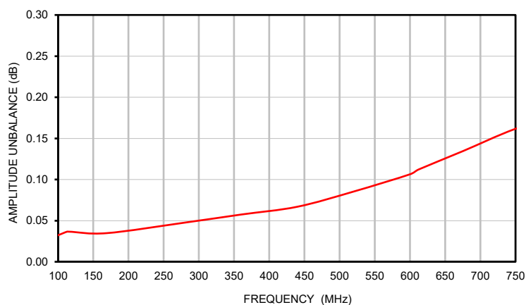
AMPLITUDE UNBALANCE
