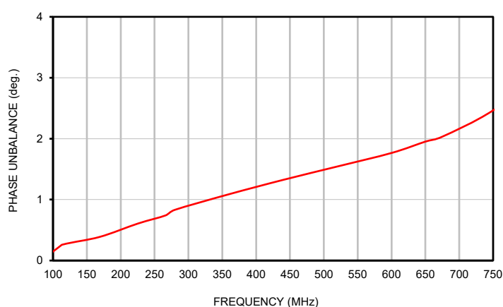
PHASE UNBALANCE
