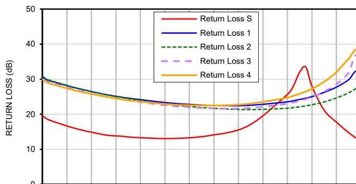
RETURN LOSS
