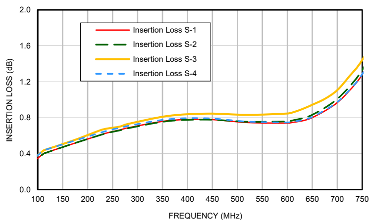
INSERTION LOSS
