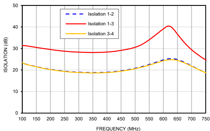
ISOLATION
