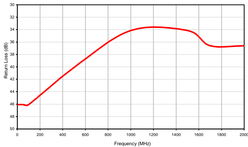
SMA-Male Return Loss
