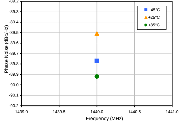
Phase Noise @ 10kHz offset (RF)
