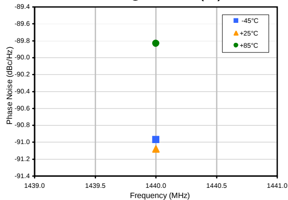
Phase Noise @ 1kHz offset (RF)
