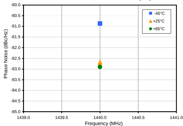
Phase Noise @ 100Hz offset (RF)
