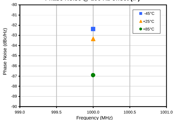
Phase Noise @ 100 Hz offset (IF)
