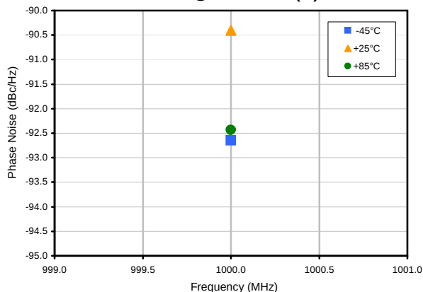
Phase Noise @ 1kHz offset (IF)
