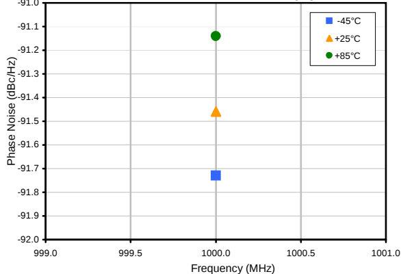
Phase Noise @ 10kHz offset (IF)
