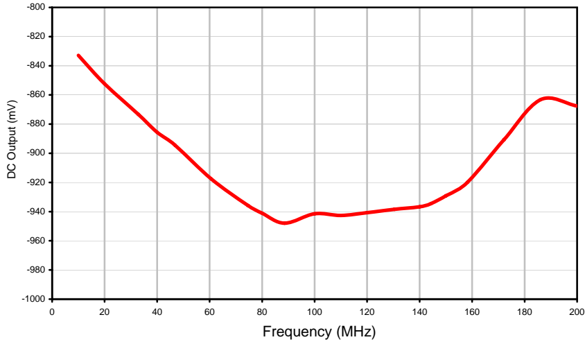
DC Offset
