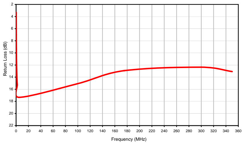
Return Loss
