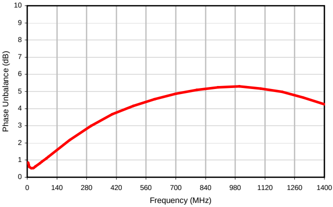
Phase Unbalance
