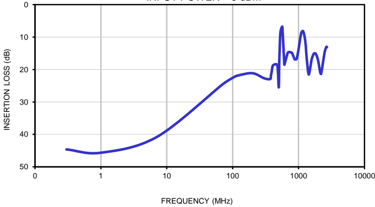
COMMONPORT RETURN LOSS INPUT POWER = 0 dBm
