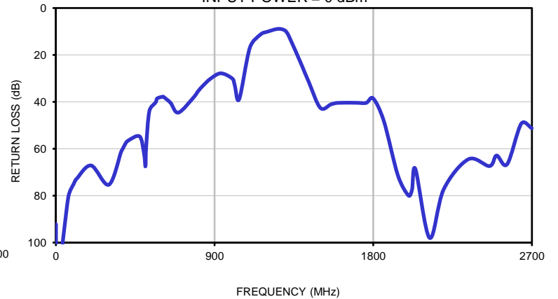
CROSSOVER ISOLATION BETWEEN BPF & HPF INPUT POWER = 0 dBm
