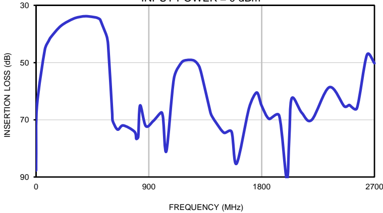
CROSSOVER ISOLATION BETWEEN LPF & HPF INPUT POWER = 0 dBm
