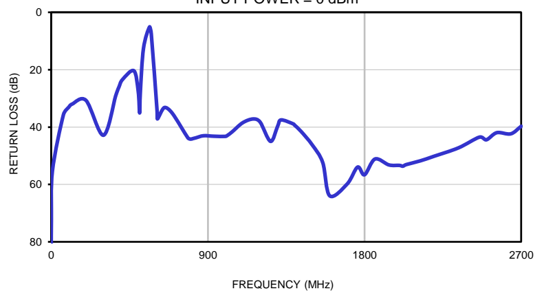
CROSSOVER ISOLATION BETWEEN LPF & BPF INPUT POWER = 0 dBm
