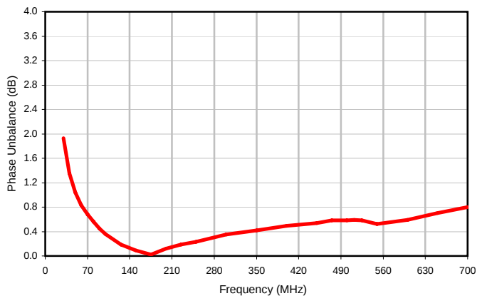
Phase Unbalance
