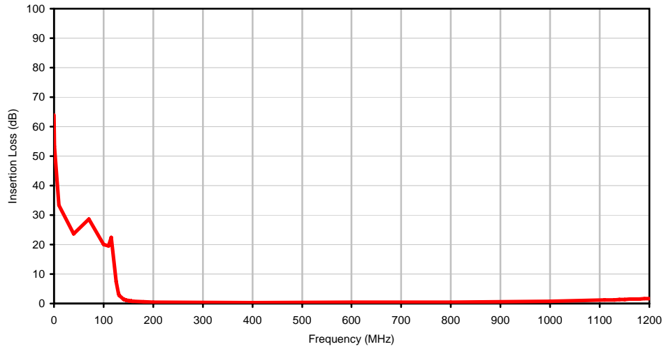
Insertion Loss
