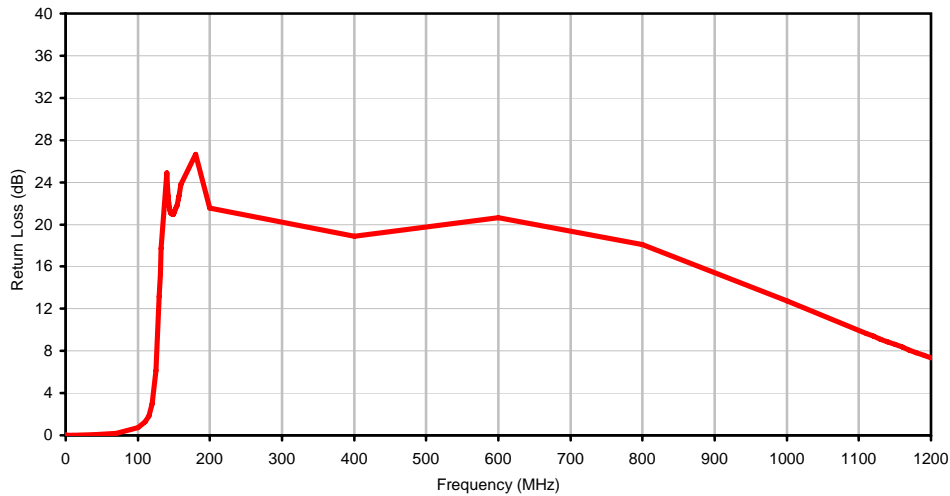
Return Loss
