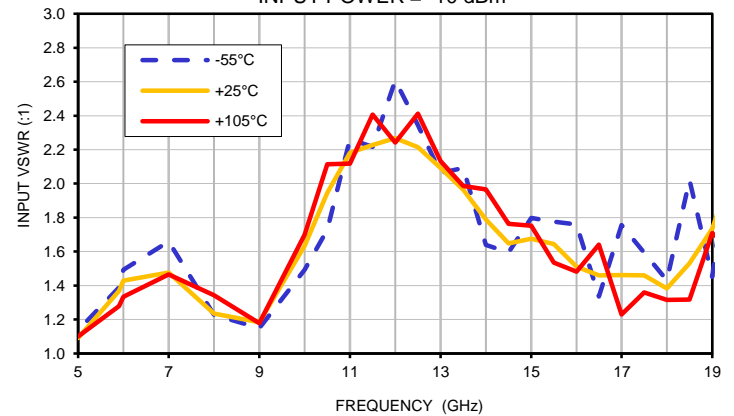
INPUT VSWR vs. TEMPERATURE (Pass Band)
