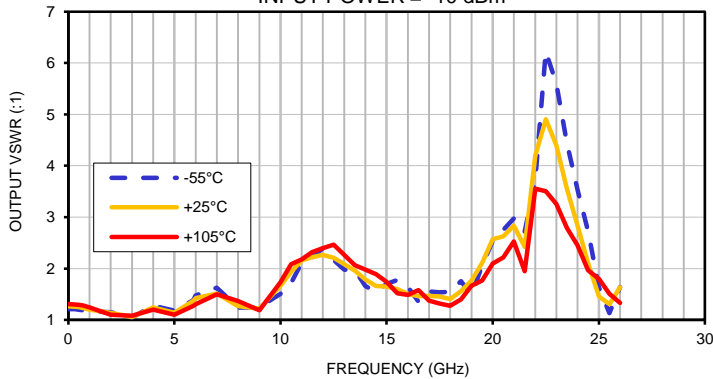
OUTPUT VSWR vs. TEMPERATURE (Full Band)
