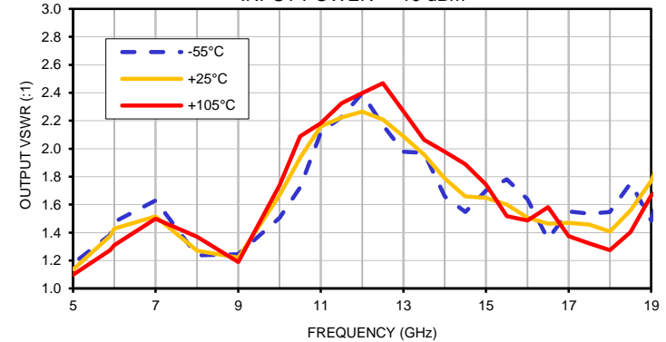
OUTPUT VSWR vs. TEMPERATURE (Pass Band)
