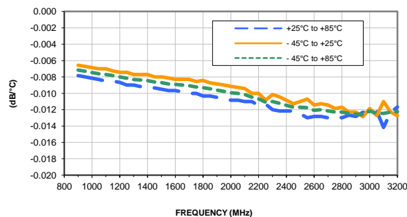
GAIN VARIATION vs. FREQUENCY & TEMPERATURE INPUT POWER = -25dBm, Vd = 5.00V
