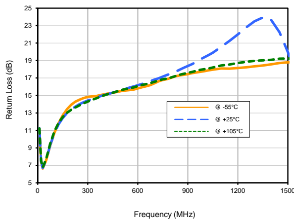
Return Loss Forward vs. TEMPERATURE
