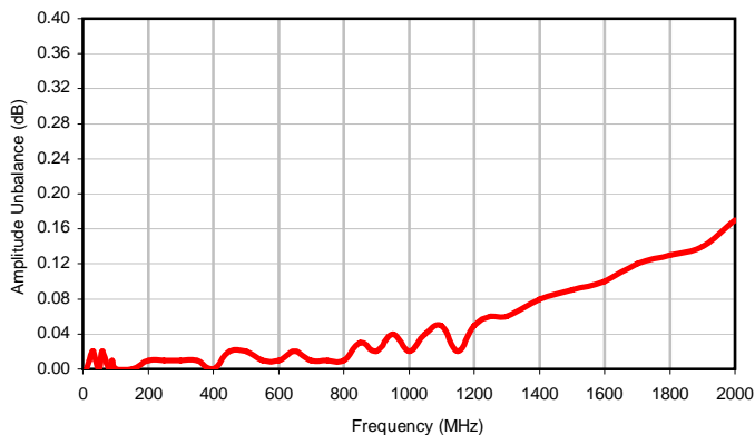
Amplitude Unbalance
