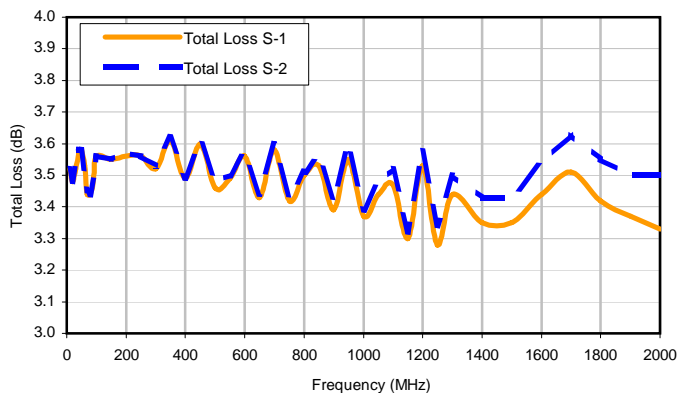
Total Loss
