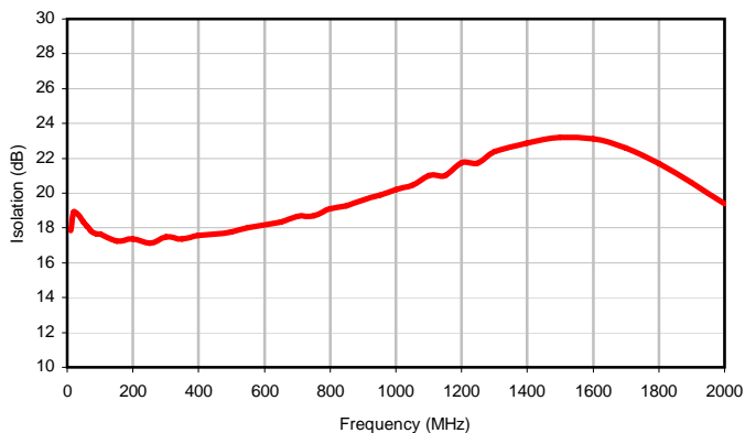
Isolation
