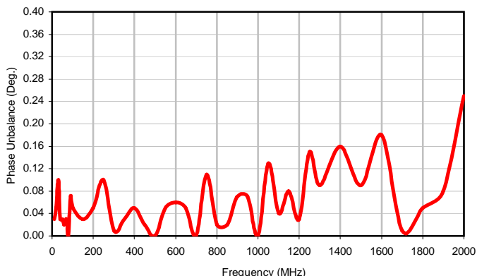
Phase Unbalance
