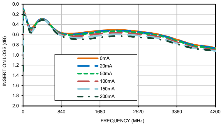
INSERTION LOSS
