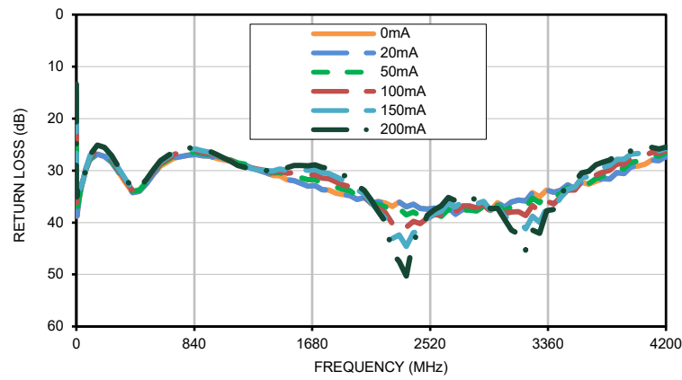
RETURN LOSS
