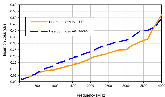
Insertion Loss
