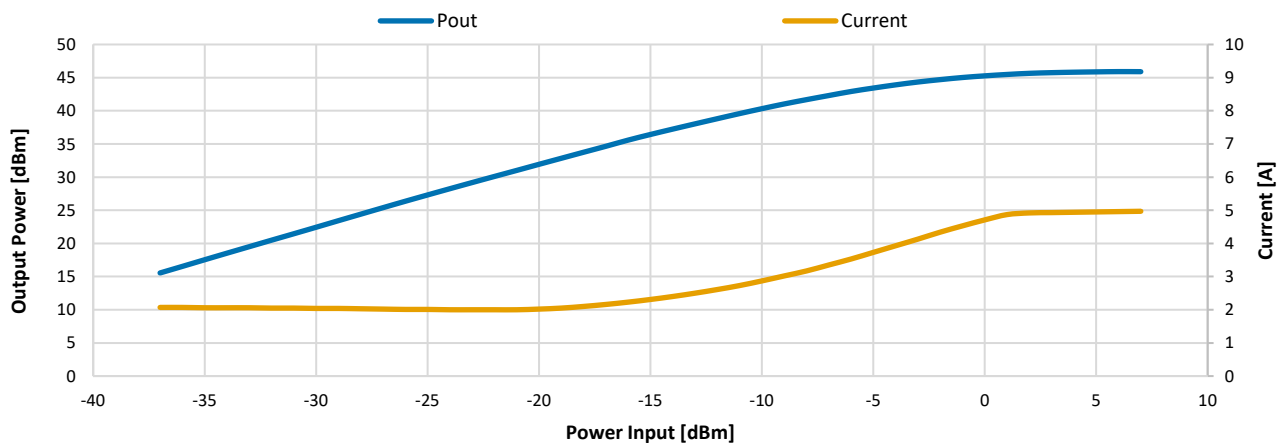
Power Out &amp; Current vs. Power In @ 5000 MHz
