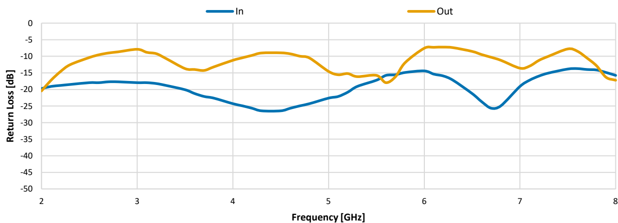
Return Loss vs. Frequency
