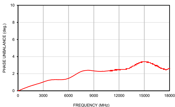
PHASE UNBALANCE
