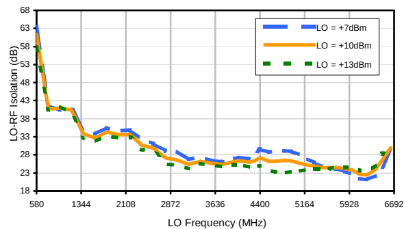
LO-IF Isolation
