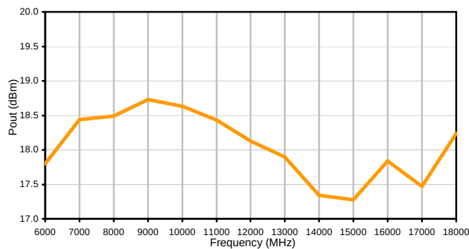
Pout @ 1dB Compression @ 5V
