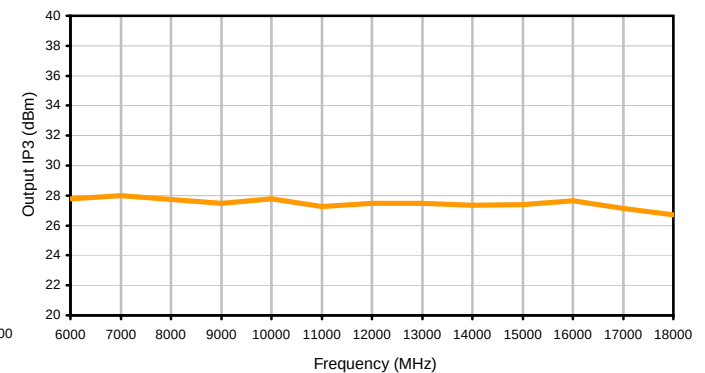
Output IP3 @ 5V
