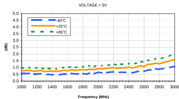
NOISE FIGURE vs. FREQUENCY & TEMPERATURE
