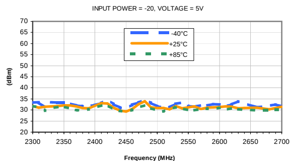
OUTPUT IP3 vs. FREQUENCY & TEMPERATURE
