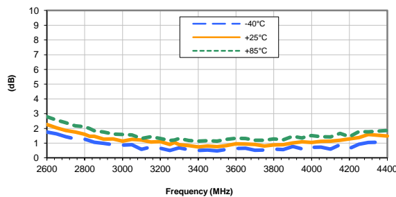
Noise Figure vs. TEMPERATURE VOLTAGE = 5V
