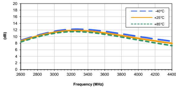
GAIN vs. TEMPERATURE INPUT POWER = -25, VOLTAGE = 5V
