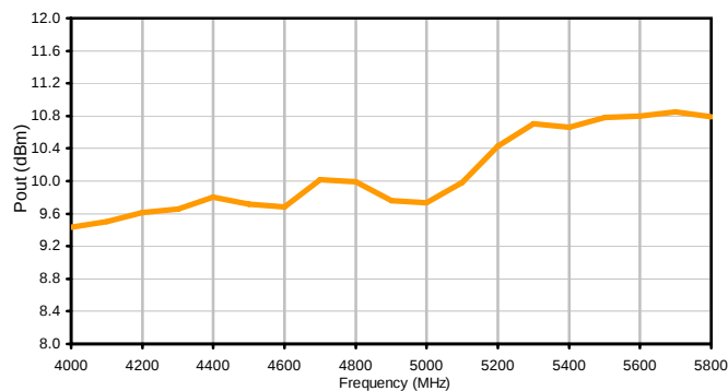
Pout @ 1dB Compression @ 12V
