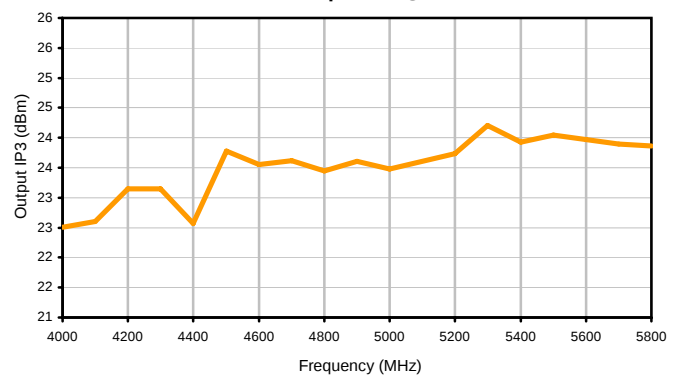
Output IP3 @ 12V
