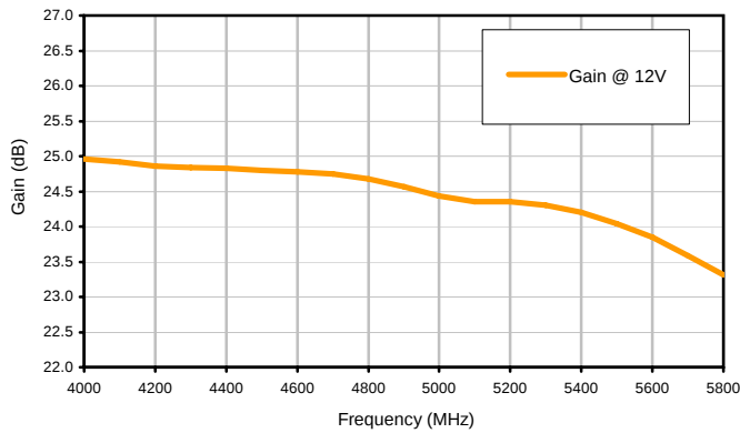
Gain
