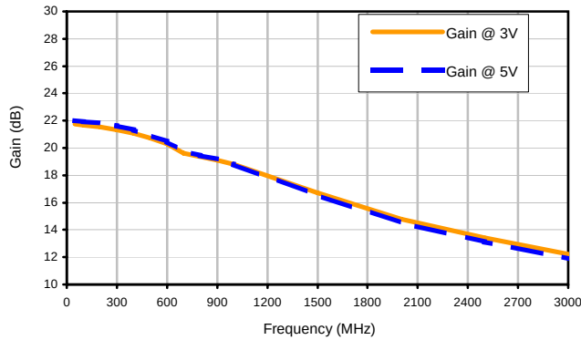
Gain
