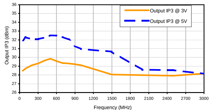
Output IP3
