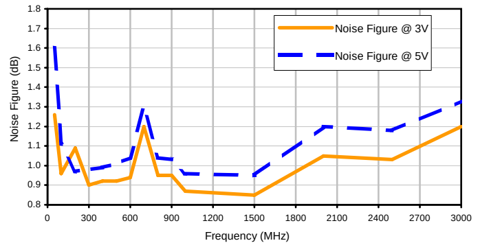
Noise Figure
